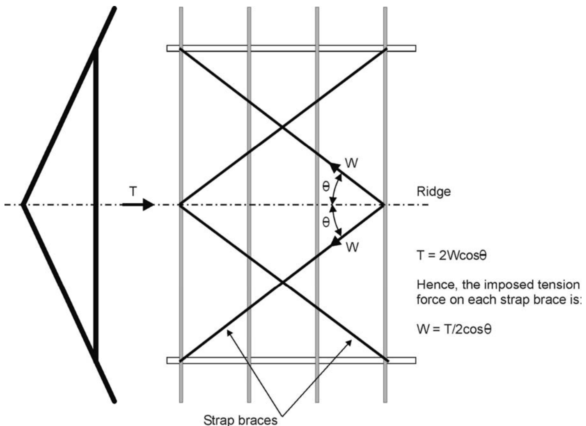
Fig. 5.4 Illustration of the relationship between a load acting along the ridge line and tension in the strap bracing
